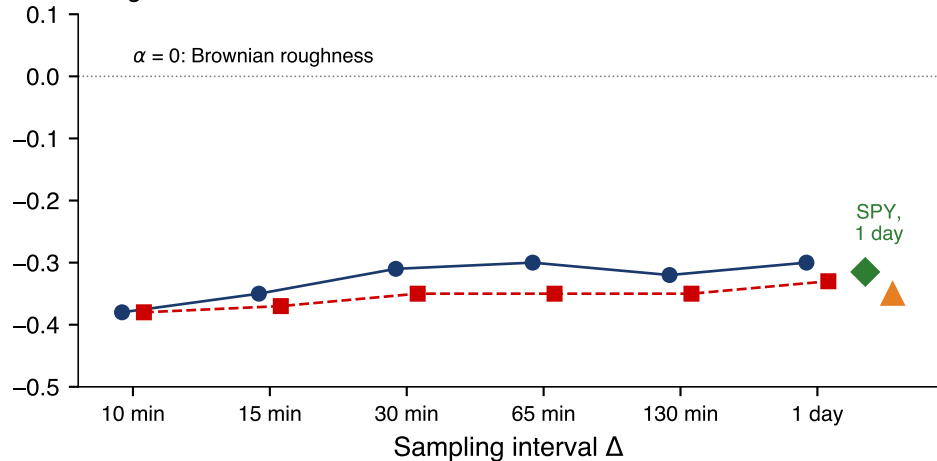
Roughness index \hat{\alpha}
