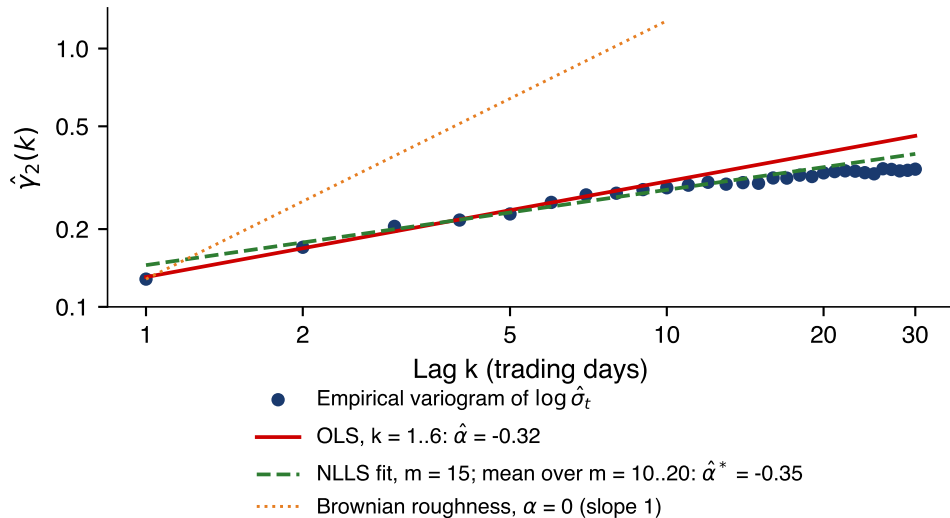
Roughness: variogram of daily log-volatility (log-log)
