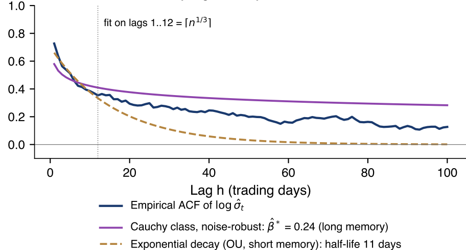
Persistence: ACF of daily log-volatility
