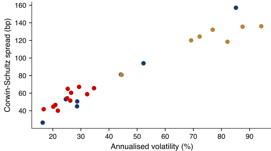
Spearman correlation 0.94
