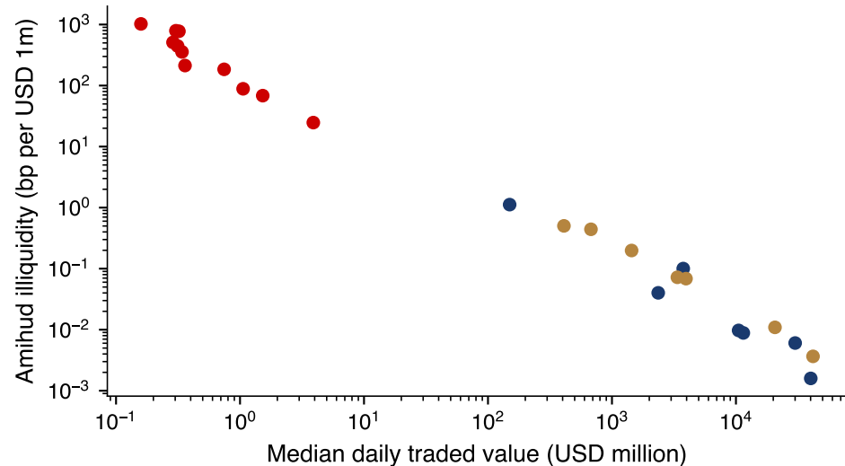
Spearman correlation -0.99
