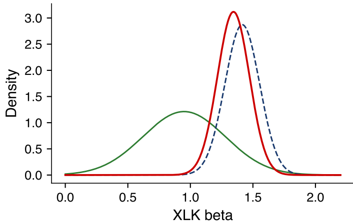
Prior x likelihood = posterior
