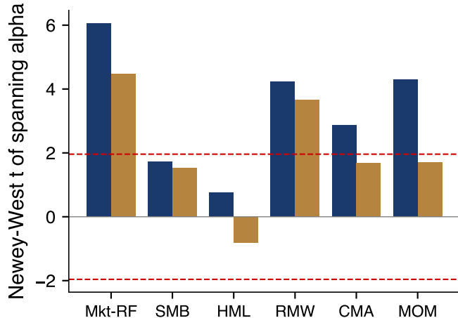
Each factor on the other five
