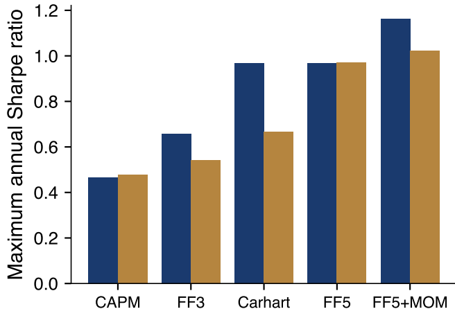
Sharpe ratio of each model's factors
