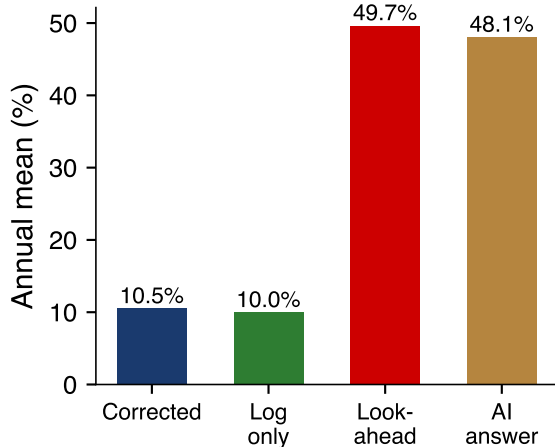
Which error does the damage?
