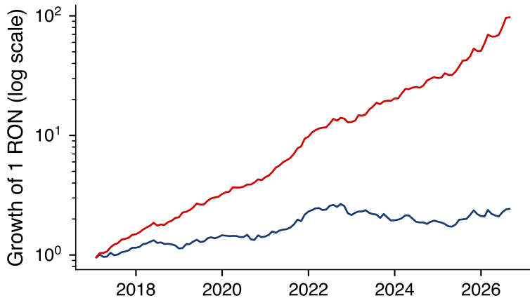
Same months, same stocks
