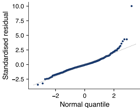
Q-Q plot
