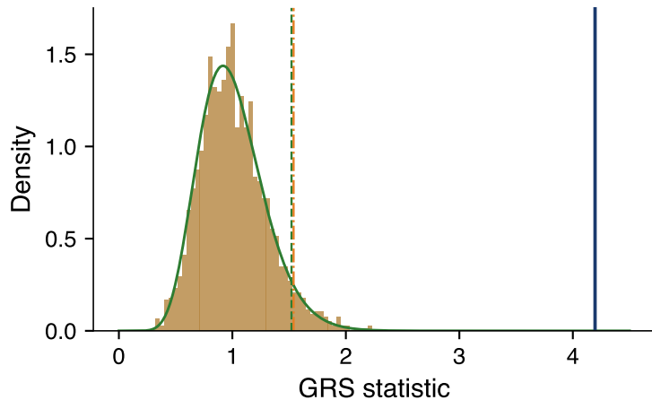
Null distribution of GRS
