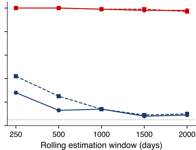
GJR-GARCH(1,1)
