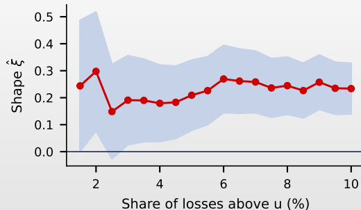
Stability of \xi across thresholds
