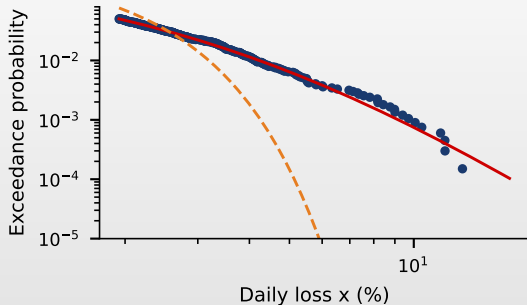
BET: largest 5% of daily losses
