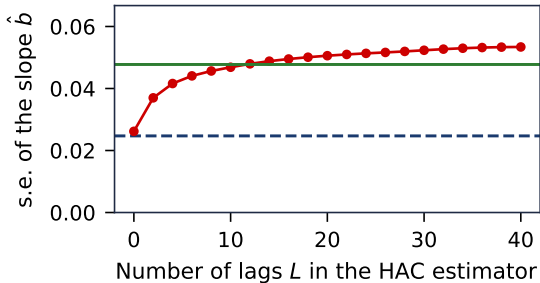
Slope standard errors, n = 1500
