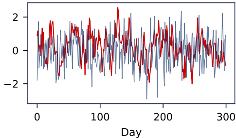
Residuals: persistent against independent
