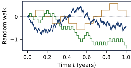
Random walk with steps \pm\sqrt{\Delta}
