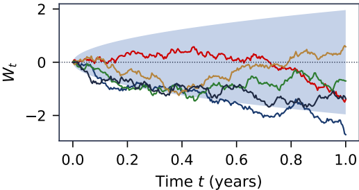
Brownian motion: W_t \sim N(0, t)
