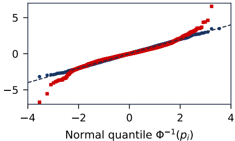
QQ plot
