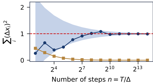
Quadratic variation as the grid is refined
