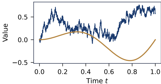
Two paths on [0, 1]
