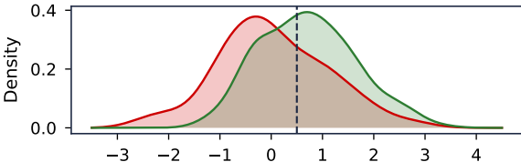
Simulated scores of the two groups
