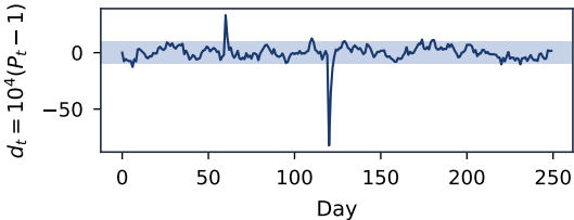
Simulated TAR: \phi_{\text{in}} = 0.9 , \phi_{\text{out}} = 0.4
