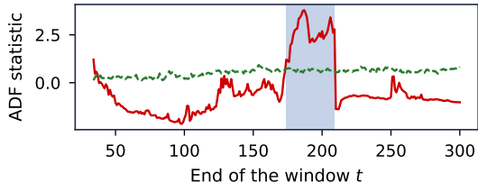
T = 300, w_0 = 34, L = 6
