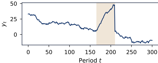
Random walk with one bubble
