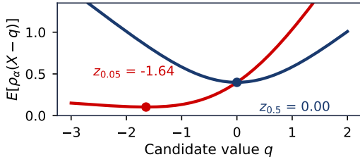
X \sim N(0, 1) : expected loss
