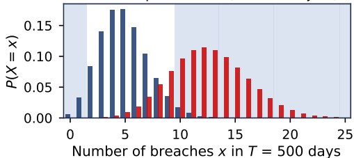
Size 0.071, power 0.80 (shaded: reject)
