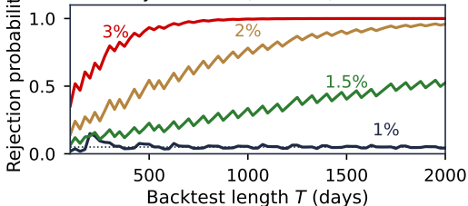
Power by true rate (1%: size)
