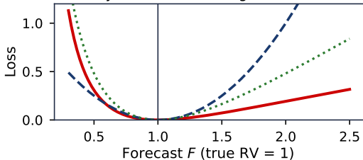
One day: under-forecasting costs more
