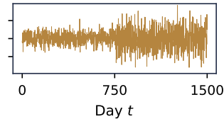
RW2: \sigma_t shifts
