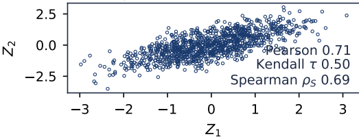
Normal pair ( Z_1, Z_2 )
