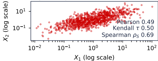
Lognormal pair ( e^{1.5Z_1}, e^{1.5Z_2} )
