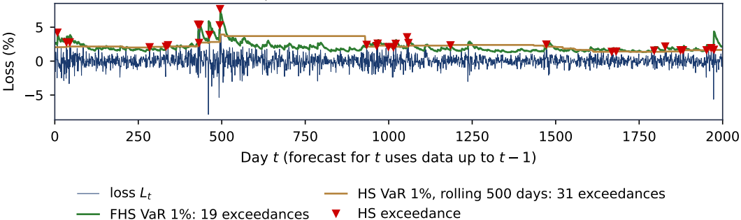
Simulated GARCH returns; expected exceedances n\alpha = 20
