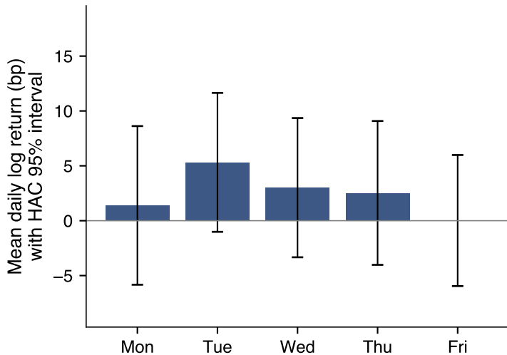
S&P 500 (US): equal-means p = 0.83
