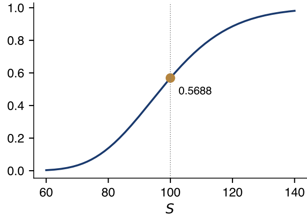
Delta \Phi(d_1)
