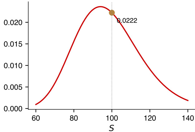
Gamma \phi(d_1)/(S\sigma\sqrt{\tau})
