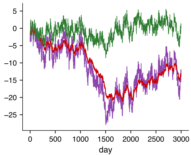
One simulated random walk
