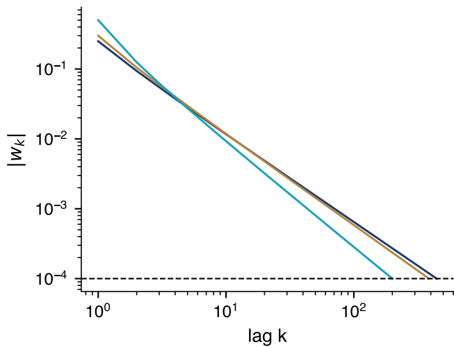
Weights, log-log scale
