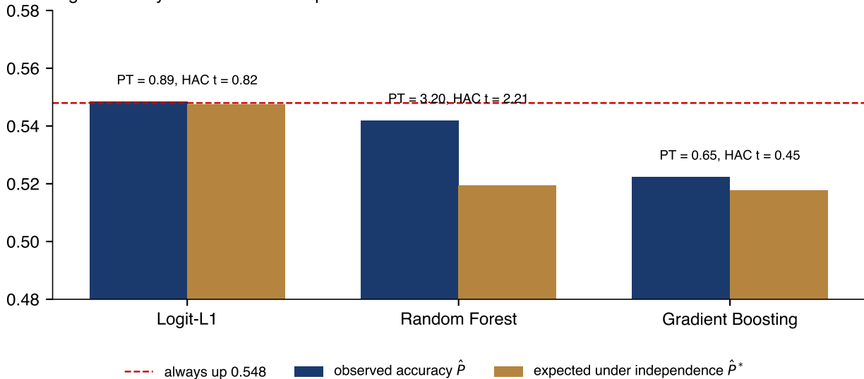
Sign accuracy: observed vs. independence benchmark
