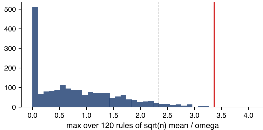
Benchmark cash: SPA p = 0.002 , StepM keeps 120
