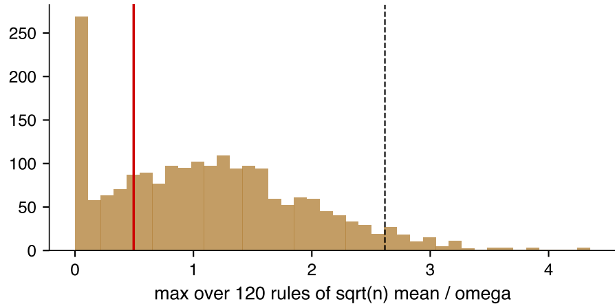
Benchmark buy-and-hold: SPA p = 0.748 , StepM keeps 0
