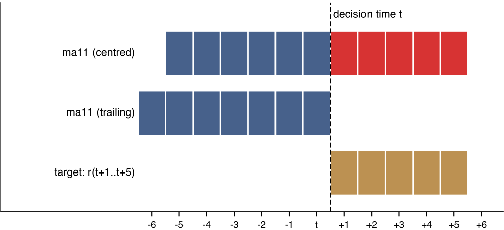
Which daily returns enter each feature on day t (trailing window shown from t-6)
