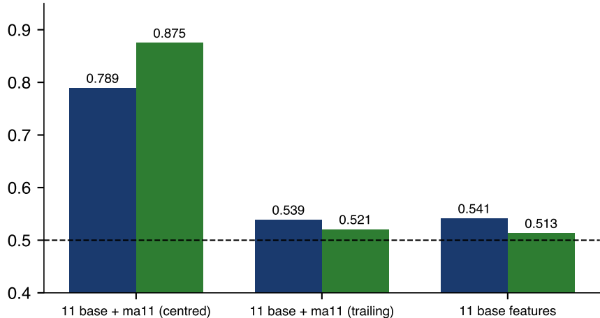
Purged 5-fold CV, BTC 5-day direction
