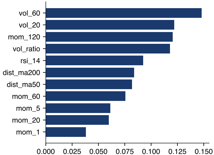
MDI (in sample)
