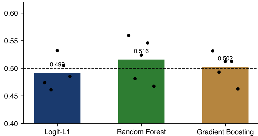
ROC AUC, mean of 5 purged folds
