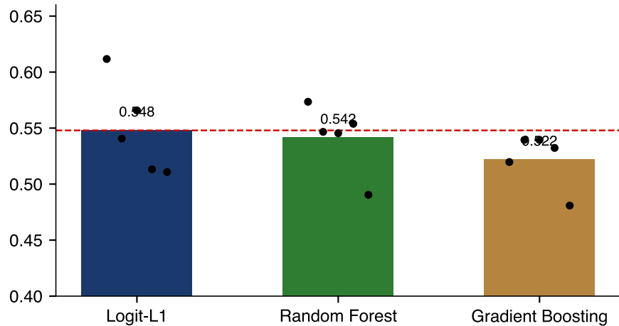
accuracy, mean of 5 purged folds
