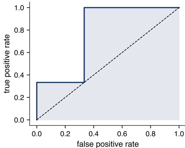
ROC staircase
