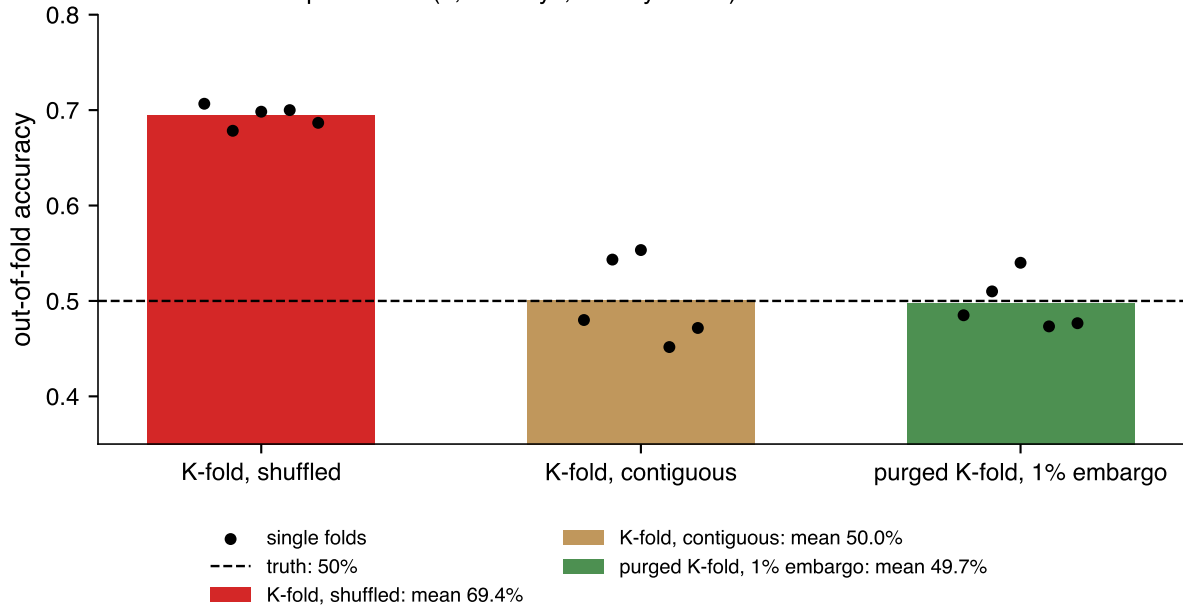
Random forest on pure noise (3,000 days, 20-day labels)
