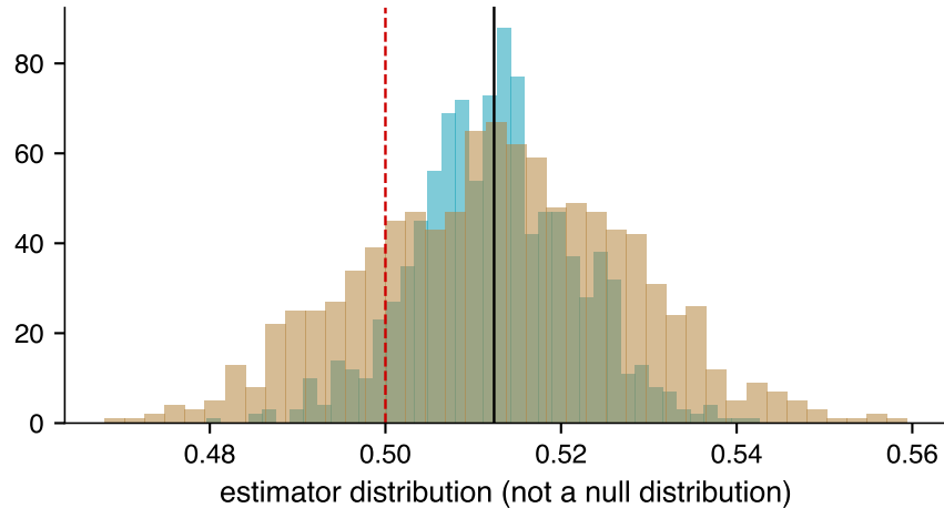
Serial dependence widens the distribution
