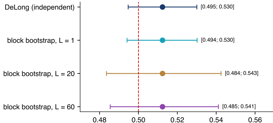
RF pooled AUC = 0.512: 95% intervals
