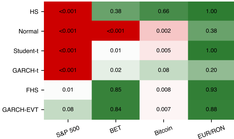
Strict ESR, two-sided p-value
