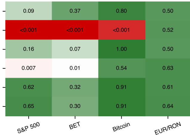
Intercept ESR, one-sided p-value
