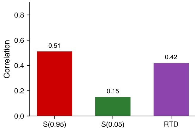
Monthly correlation with CATFIN (Figure 13)
