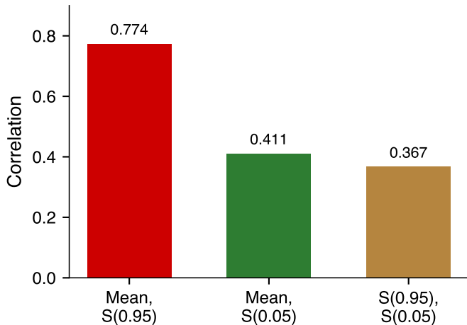
Rolling 250-day indices (Table 3)
