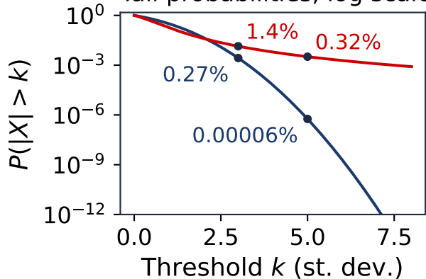
Tail probabilities, log scale
