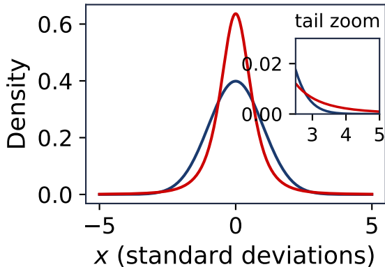
Densities, same variance
