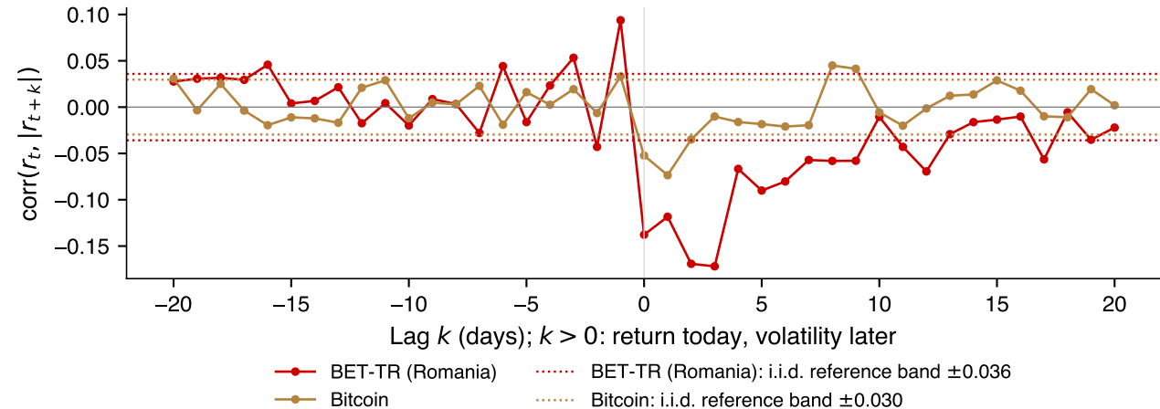
Leverage effect: Romania (BET-TR) vs crypto (Bitcoin)
