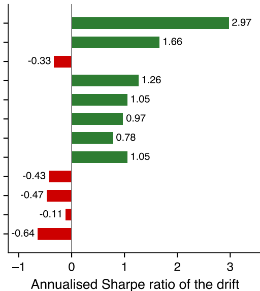
Is the drift profitable?
