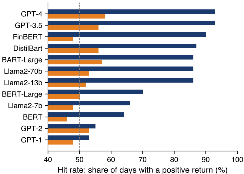
Does the long-short portfolio point the right way?
