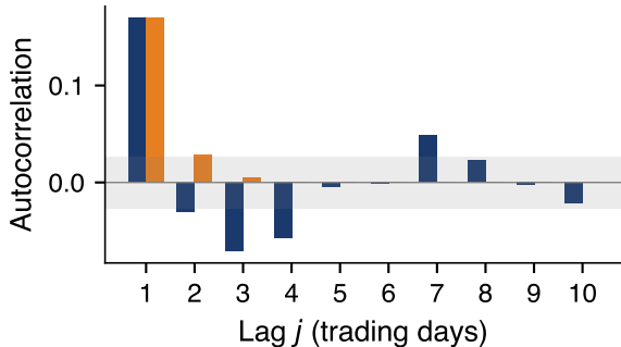
Autocorrelation of daily log changes
