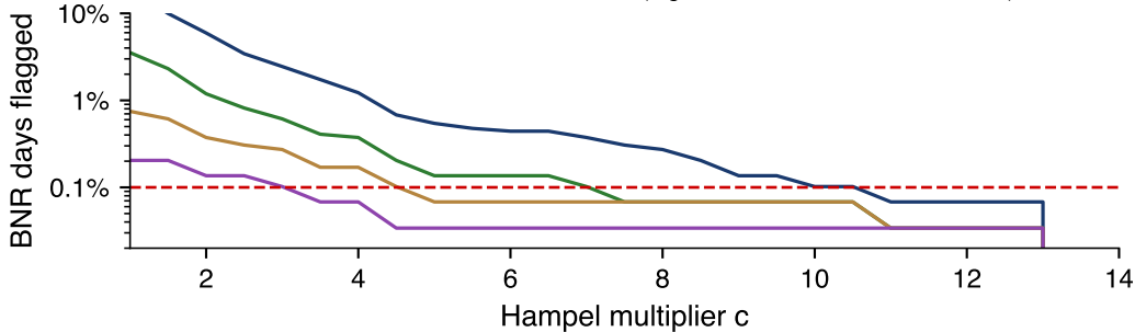
False-alarm rate on the BNR series, 2015-2026 (log scale; a zero rate is not drawn)
