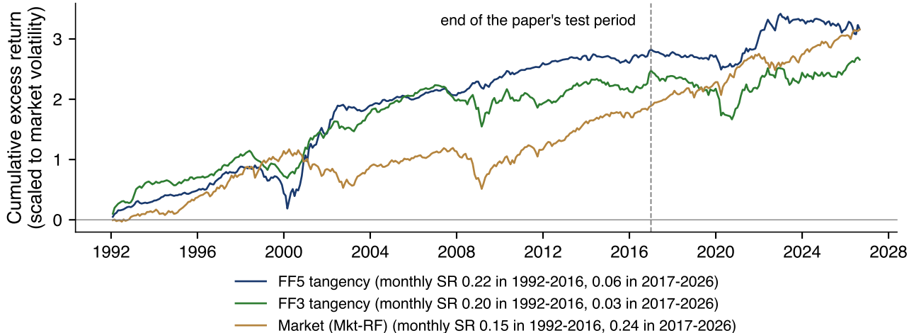
Tangency portfolios with weights fixed on 1967-1986: Jan 1992 - Aug 2026
