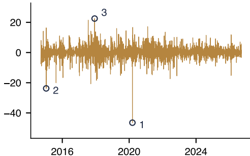
Bitcoin: daily log return (%)
