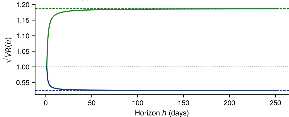
Illustrative AR(1) calculation: correction factor of the \sqrt{h} rule
