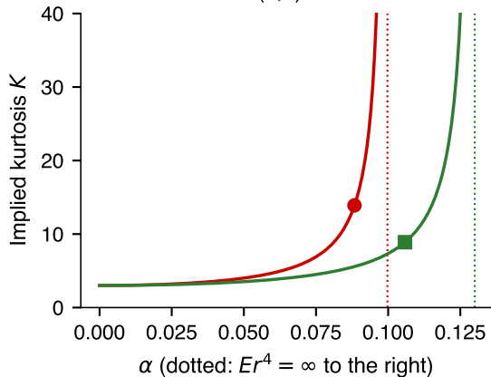
Gaussian GARCH(1,1): kurtosis vs \alpha
