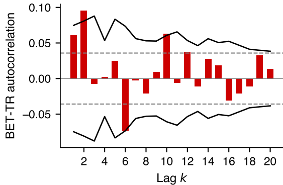
Returns r_t : is the direction predictable?
