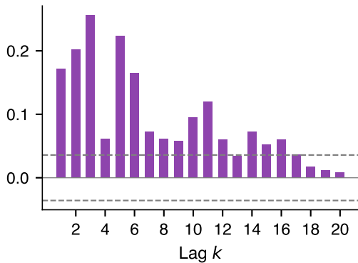
Squares r_t^2 : does volatility cluster?
