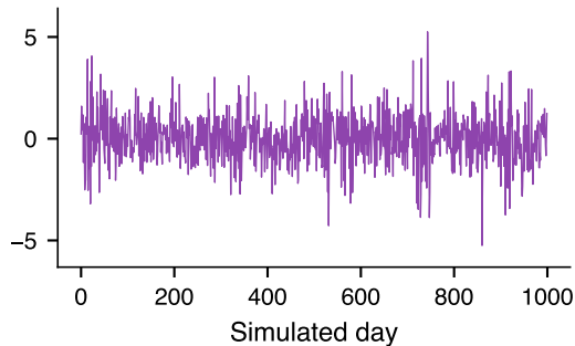
A8: persistent Markov regimes
