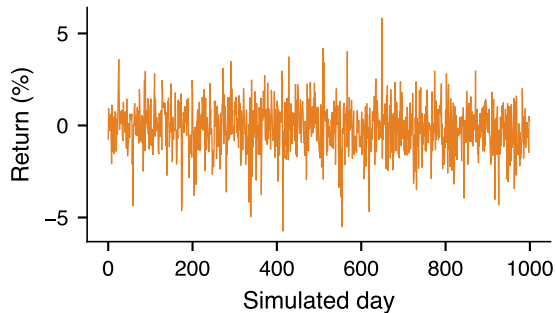
A6: volatility state drawn independently each day
