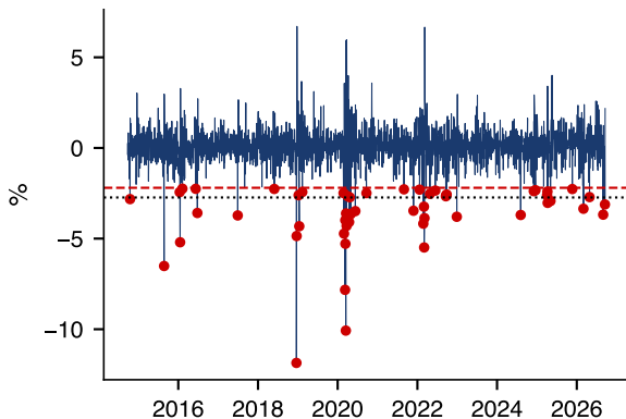
Breaches over time (in-sample)
