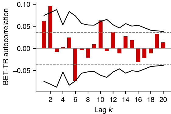
Returns r_t : is the direction predictable?
