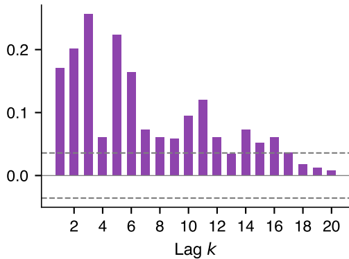
Squares r_t^2 : does volatility cluster?
