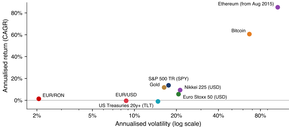
Risk and return, 2015-2026: assets in USD, EUR/RON in RON per EUR
