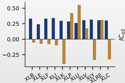
Eigenvector loadings
